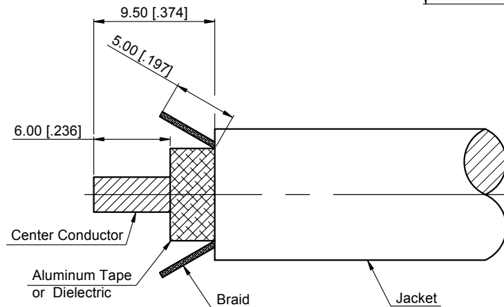
Cable Stripping Dimensions
