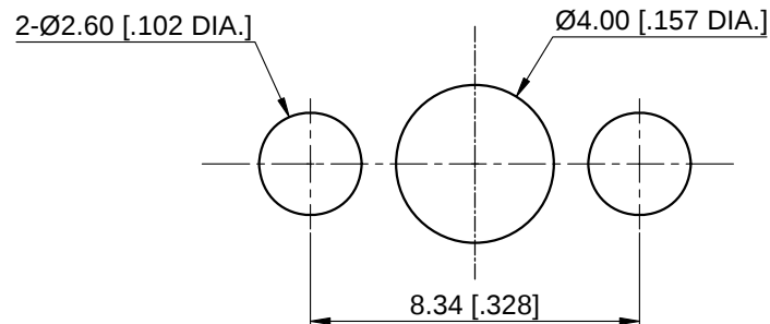
Recommended Mounting Holes
