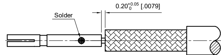
PIN CONTACT SOLDERING DIMENSION
