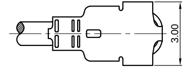
U.FL/MHF Plug Enlarged Drawing 6:1
