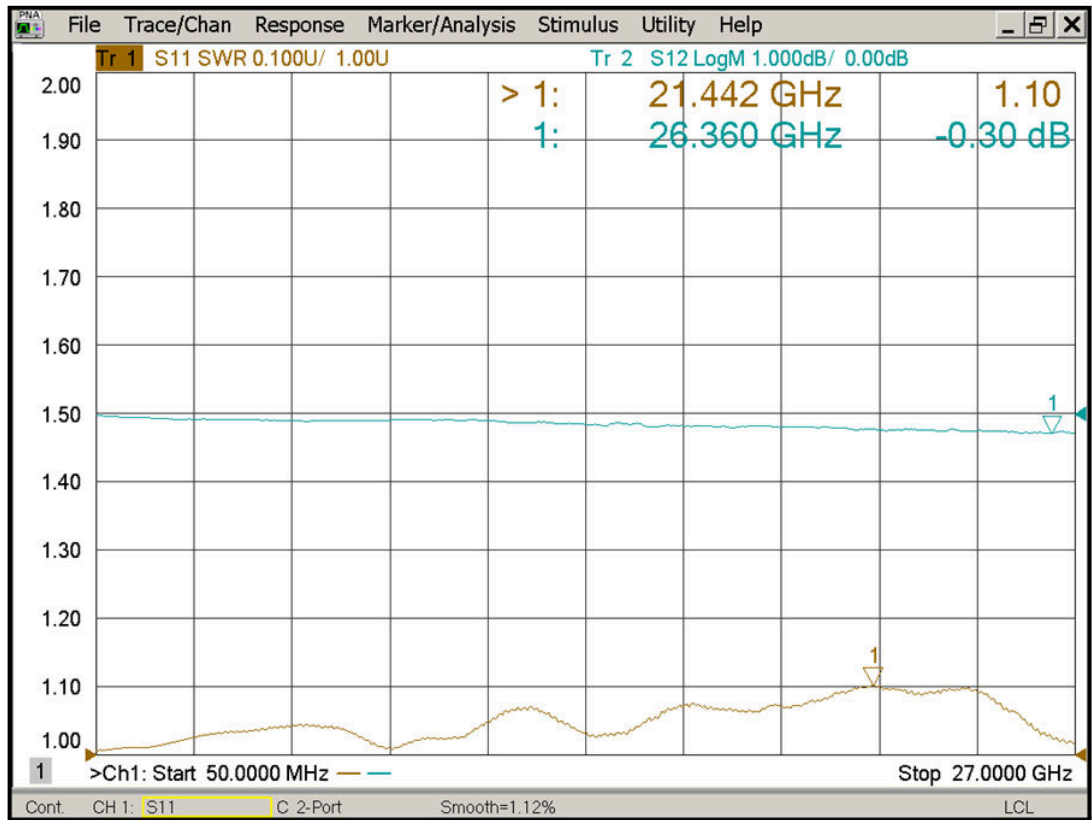
P-SMAM-2.92F-157 Test Report
