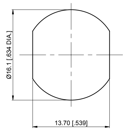
Recommend Mounting Hole
