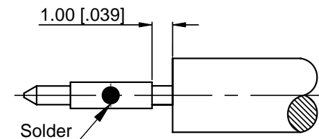
PIN CONTACT SOLDERING DIMENSION
