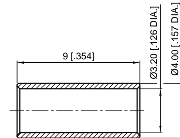
1. CRIMP FERRULE HEX. CRIMP TOOL SIZE: 3.25 [.128]
