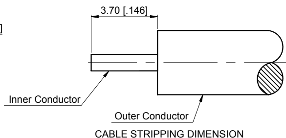
CABLE STRIPPING DIMENSION
