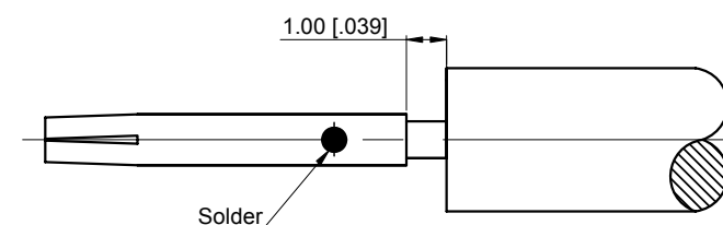
PIN CONTACT SOLDERING DIMENSION
