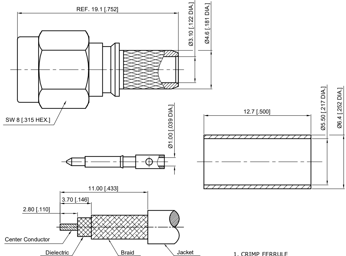
Recommended Cable Stripping Dimensions
