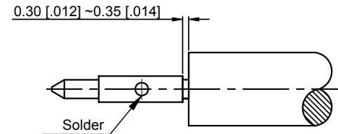
PIN CONTACT SOLDERING DIMENSION
