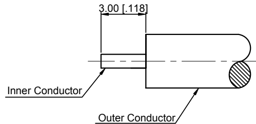
CABLE STRIPPING DIMENSION
