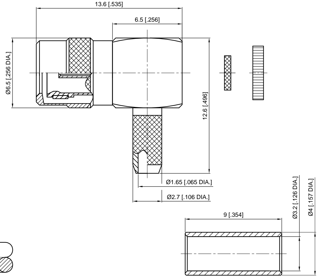
1. CRIMP FERRULE HEX. CRIMP TOOL SIZE: 3.25 [0.128].
