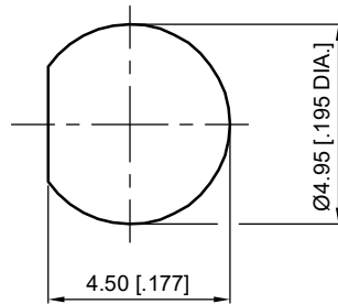
Recommended Mounting Holes
