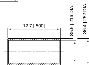
1. CRIMP FERRULE HEX. CRIMP TOOL SIZE : 5.4 [.213]
